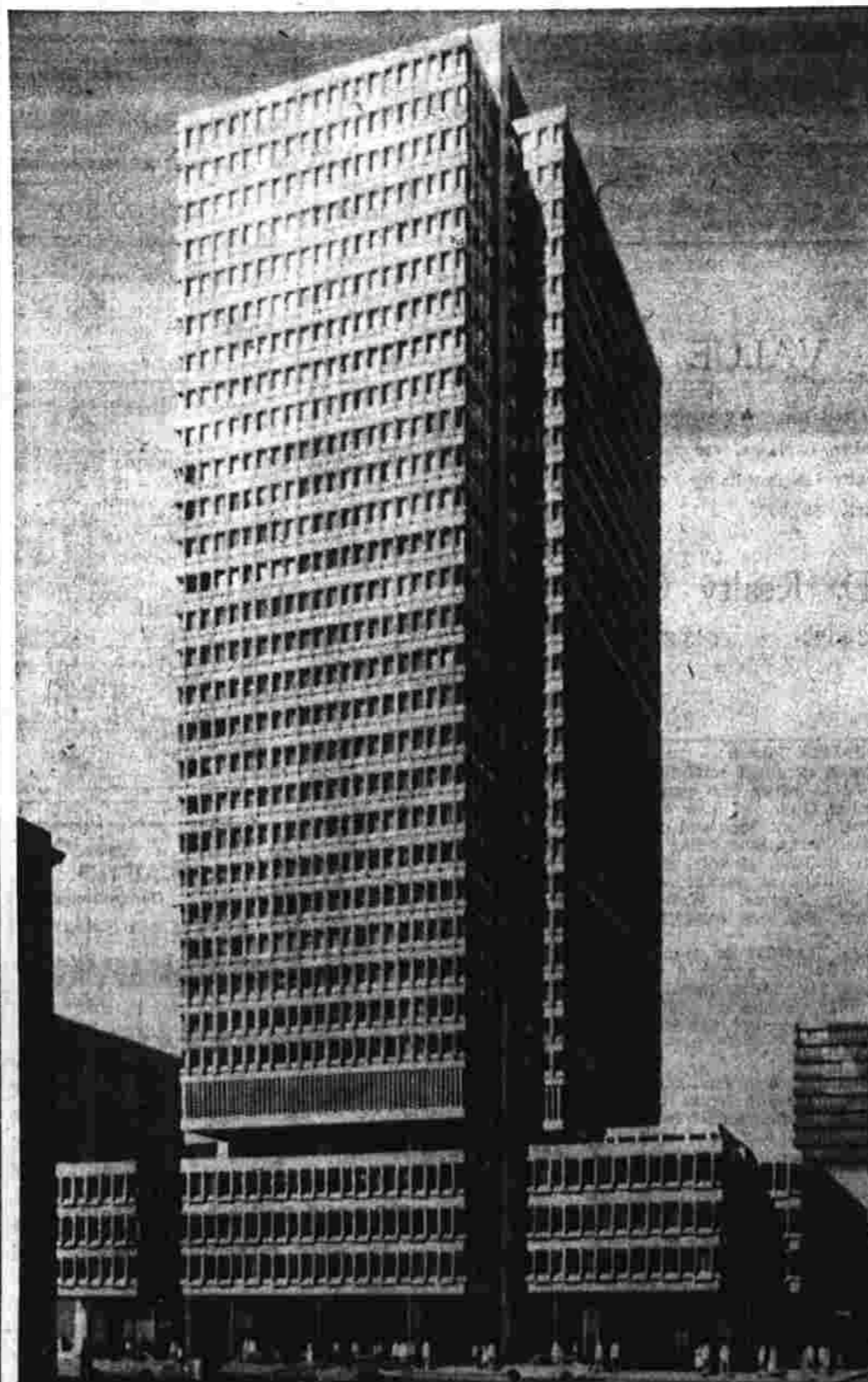
This towering structure, at 478 feet the second tallest structure in the world to be sheathed entirely in pre-cast concrete panels, has had all its concrete components composed in Manchester. This week a young Manchester firm is sending off its last shipment of the more than 8,000 separate sections of pure quartz aggregate which form the building block muscles of the colossus — the new State Street Bank in Boston. Born about four years ago as the pre-cast division of the Glaxon Corp., the Allied Casting Corporation at 260 Tolland Tpk. recently became a separate corporation under the management of Roy E. Chasse of South Windsor, who also serves as the vice president of the firm. At first utilizing a small plant with a dozen employees, the firm, specializing in textured concrete architectural elements, has since expanded to what Chasse calls an optimum size and now employs more than 100 persons. Besides its contribution to the Boston skyline, Allied Casting has also sculptured the greatest portion of the buildings and walkways at Constitution Plaza in Hartford and much of the stonework of the sculpture and arts buildings of the University of Hartford. (Herald photo by O'Brien.)
